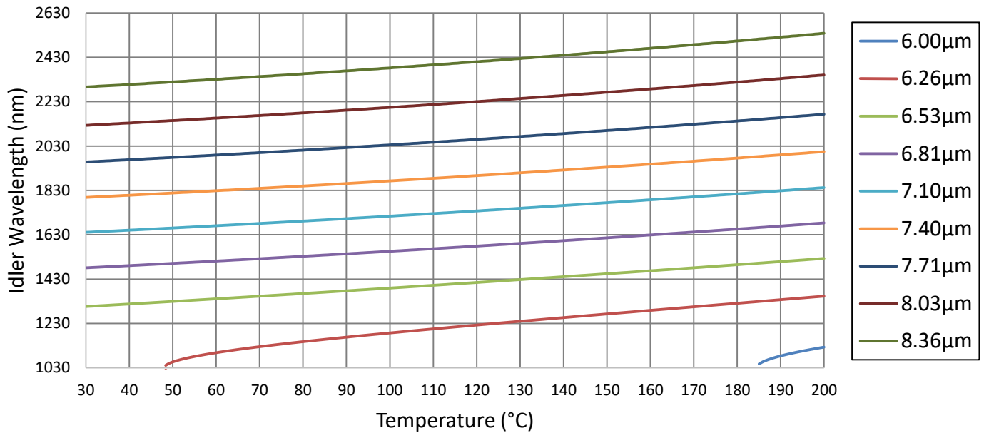
OPO Tuning Curve 515nm Pump
